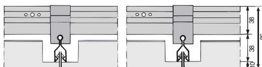
Clip-in profile
