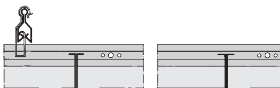
Primary suspension
