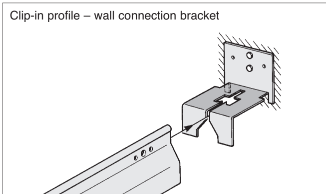
Clip-in profile – splice
